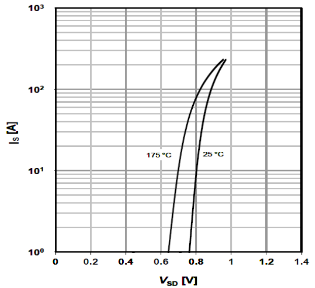
IS -- VSD
